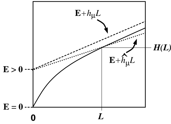
FIG. 19. Assumed synchronization converted to false predictability: Schematic illustration of how assuming one is synchronized to a process, leads to an underestimate \widehat{h}_\mu for a source with excess entropy \mathbf{E} > 0 and entropy rate h_\mu .
