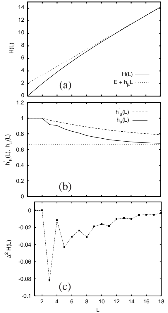
FIG. 9. (a) Entropy growth (solid line) for the random-random-XOR process, along with the asymptote \mathbf{E} + h_\mu L (dotted line). (b) Entropy convergence, both h_\mu(L) (solid line) and h'_\mu(L) (dashed line), for the same. (c) Predictability gain \Delta^2 H(L) versus sequence length.
