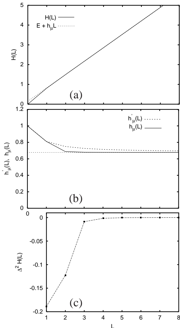
FIG. 13. (a) Entropy growth (solid line) for the simple nondeterministic source, along with the asymptote \mathbf{E} + h_\mu L (dashed line). (b) Entropy convergence, both h_\mu(L) (solid line) and h'_\mu(L) (dashed line), for the same. (c) Predictability gain \Delta^2 H(L) versus sequence length.
