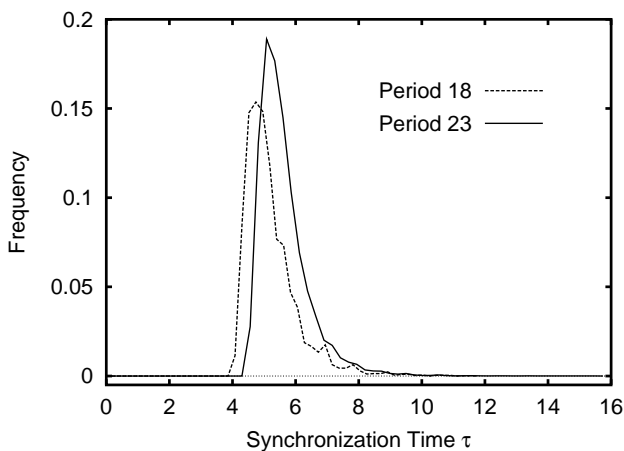
FIG. 8: Normalized histogram of the distribution of \tau values for period-18 and period-23 sequences.
