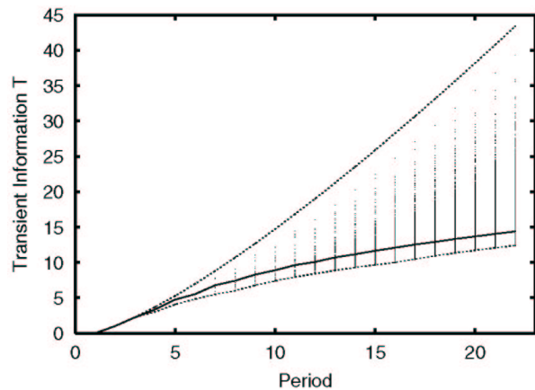
FIG. 4: Scatter plot of the transient information \mathbf{T} for all distinct periodic sequences as a function of their prime period P , up to P = 22 . The dashed lines are the maximum and minimum \mathbf{T} values computed analytically; see text. The solid line gives the estimated average \mathbf{T} value at the given period.
