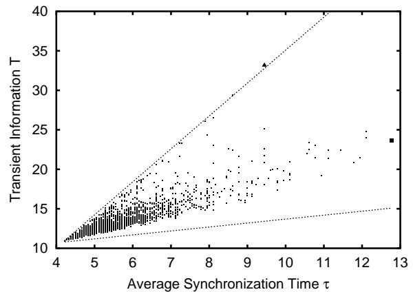
FIG. 11: A scatter plot of \mathbf{T} versus \tau for all period-18 sequences. The upper bound is that of Eq. (48) and the lower bound is that of Eq. (50). The solid triangle is the (\tau, \mathbf{T}) point for the \mathbf{T}_{\max} sequence; the solid square denotes the \tau_{\max} sequence.
