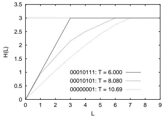
FIG. 2: Shannon entropy growth curves H(L) for three different period-8 sequences: 00010111, 00010101, and 00000001.
