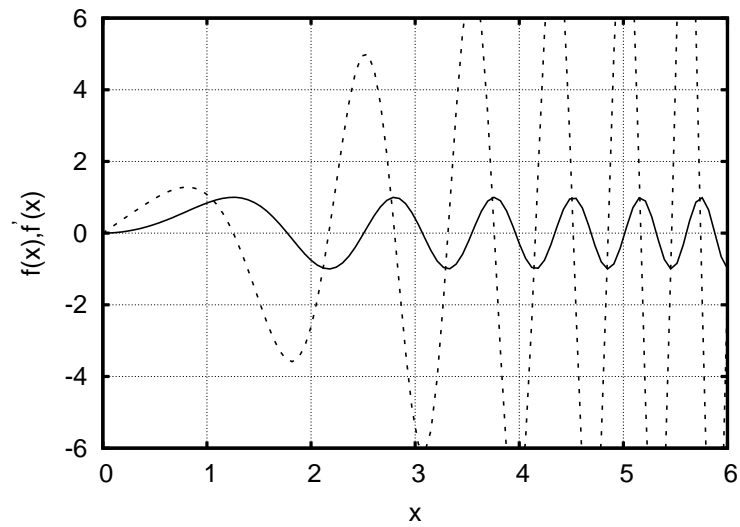
Figure 2: A plot of \sin(x^2) and its derivative, 2x\cos(x^2) .
