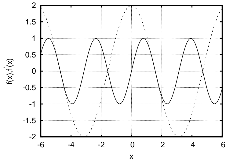
Figure 1: A plot of \sin(2x) and its derivative, 2\cos(x) .
