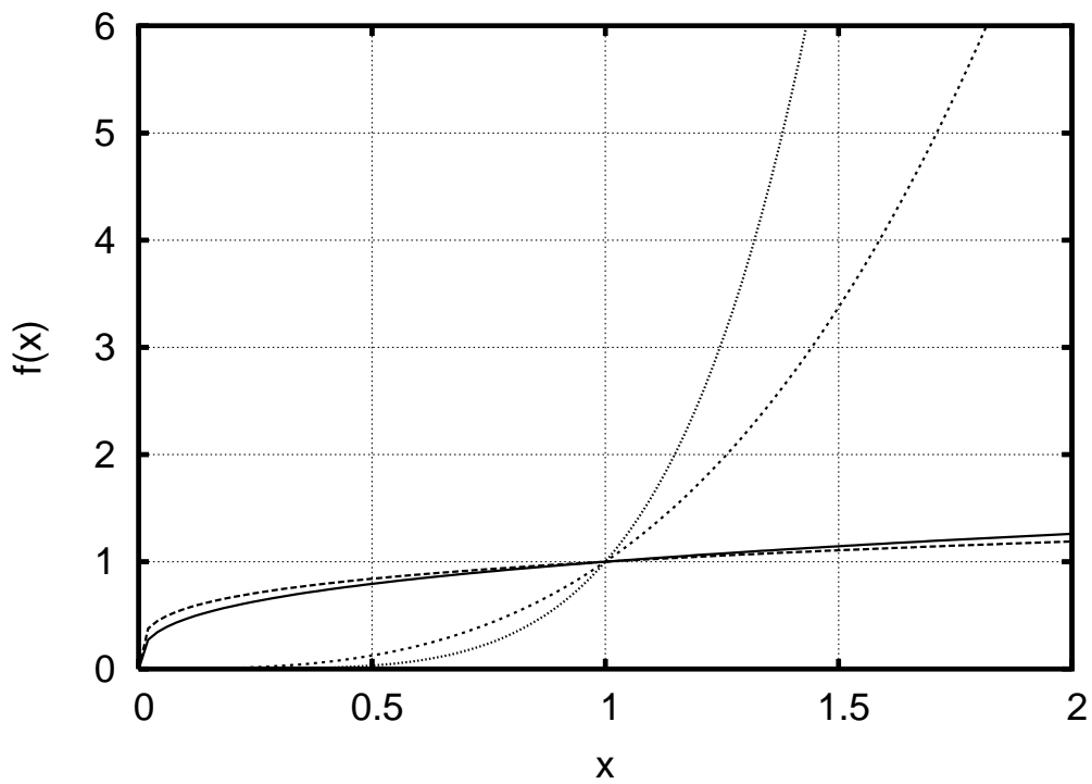
Figure 4: Plots of x^{1/3} , x^{1/4} , and x^3 , x^5 .
