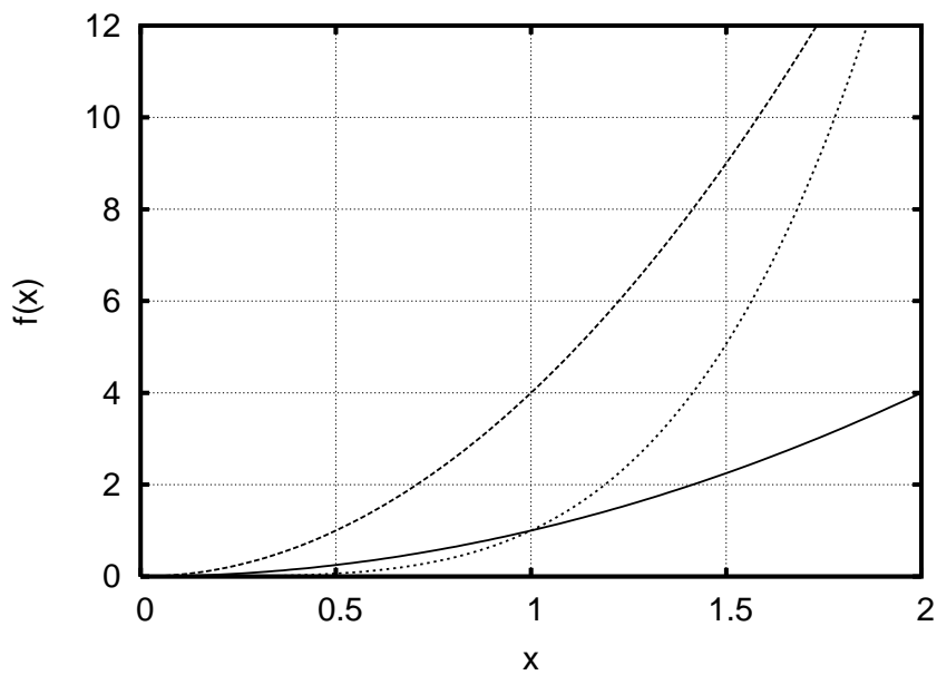
Figure 2: Plots of x^2 , 4x^2 , and x^4
