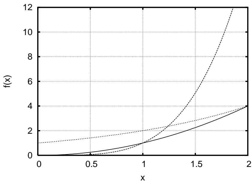
Figure 1: Plots of x^2 , x^4 , and 2^x
