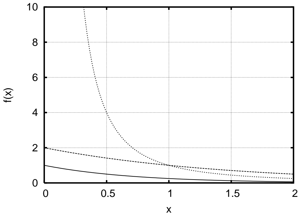
Figure 3: Plots of 2^{-2x} , 2(2^{-x}) , and x^{-2}
