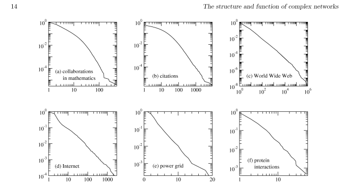
FIG. 6 Cumulative degree distributions for six different networks. The horizontal axis for each panel is vertex degree k (or in-degree for the citation and Web networks, which are directed) and the vertical axis is the cumulative probability distribution of degrees, i.e., the fraction of vertices that have degree greater than or equal to k . The networks shown are: (a) the collaboration network of mathematicians [182]; (b) citations between 1981 and 1997 to all papers cataloged by the Institute for Scientific Information [351]; (c) a 300 million vertex subset of the World Wide Web, circa 1999 [74]; (d) the Internet at the level of autonomous systems, April 1999 [86]; (e) the power grid of the western United States [416]; (f) the interaction network of proteins in the metabolism of the yeast S. Cerevisiae [212]. Of these networks, three of them, (c), (d) and (f), appear to have power-law degree distributions, as indicated by their approximately straight-line forms on the doubly logarithmic scales, and one (b) has a power-law tail but deviates markedly from power-law behavior for small degree. Network (e) has an exponential degree distribution (note the log-linear scales used in this panel) and network (a) appears to have a truncated power-law degree distribution of some type, or possibly two separate power-law regimes with different exponents.
