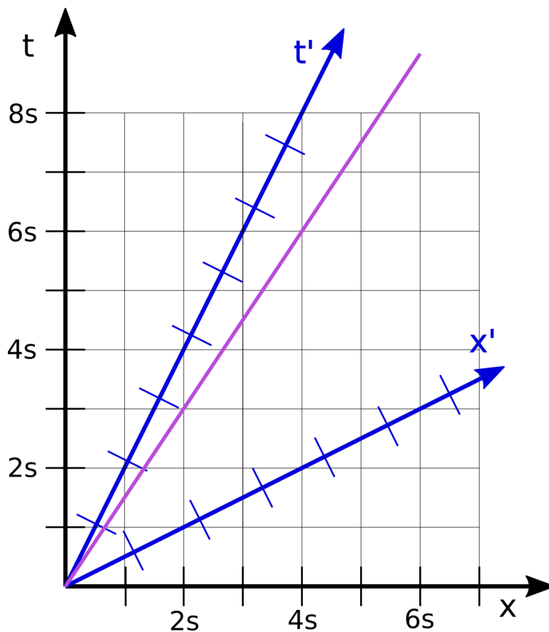
Figure 3: A spacetime diagram.
